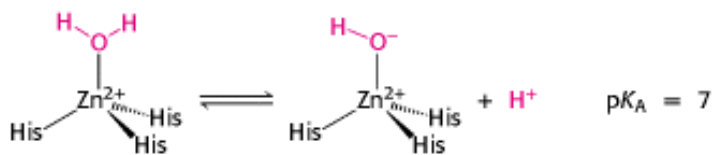
Figure 9.24. The pK_A of Water-Bound Zinc. Binding to zinc lowers the pK_A of water from 15.7 to 7.
