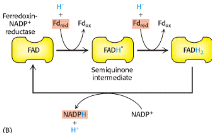
Figure 19.23. Structure and Function of Ferredoxin-NADP + Reductase. (A) Structure of ferredoxin-NADP + reductase. This enzyme accepts electrons, one at a time, from ferredoxin (shown in orange). (B) Ferredoxin-NADP + reductase first accepts one electron from reduced ferredoxin to form a flavin semiquinone intermediate. The enzyme then accepts a second electron to form FADH 2 , which then transfers two electrons and a proton to NADP + to form NADPH.
