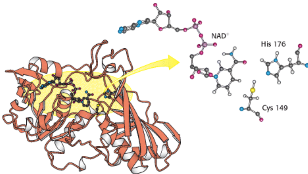
Figure 16.7. Structure of Glyceraldehyde 3-Phosphate Dehydrogenase. The active site includes a cysteine residue and a histidine residue adjacent to a bound \text{NAD}^+ .
