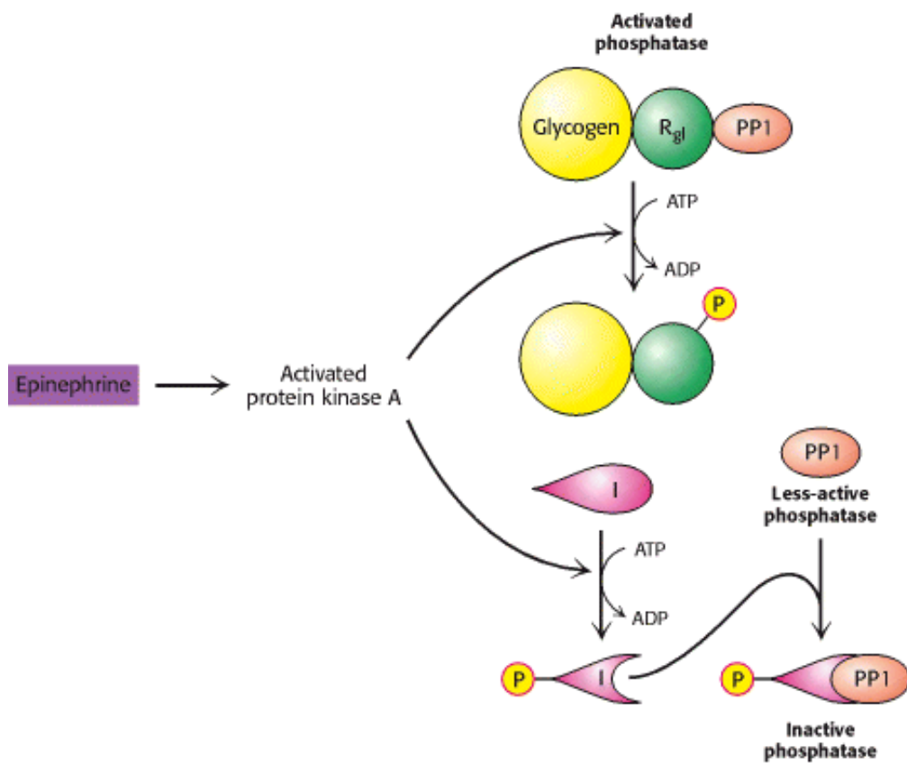
Figure 21.19. Regulation of Protein Phosphatase 1 (PP1). Phosphorylation of R GI by protein kinase A dissociates the catalytic subunit from the glycogen particle and hence the PP1 substrates. Inhibition is complete when the inhibitor subunit (I) is phosphorylated and binds to PP1 to inactivate it.
